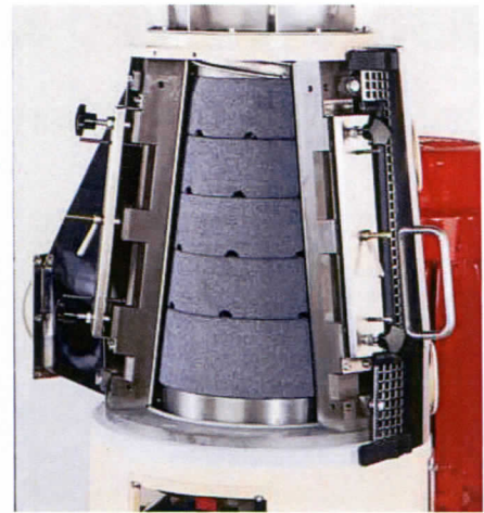
Shelling rotor
